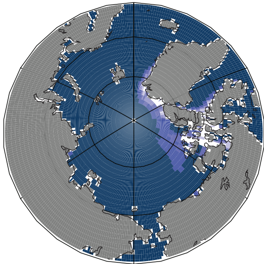
Future "ice-free" Arctic marine environment
